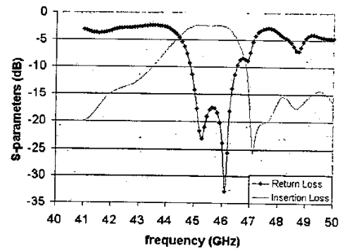
Fig. 10 Simulated performance of micromachined filter
