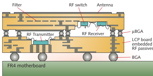
Figure 1. 3-D integrated module concept view.
