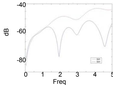
Fig. 4. Simulated S31 and S41 for a particular geometry
