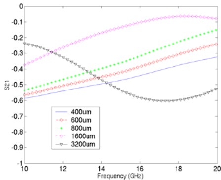
Fig. 2(a). S21 for various central line widths
