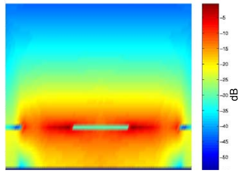
Fig. 2(b). E-field distribution
