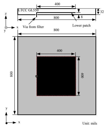
Fig. 7. Packaging adaptive stacked-patch antenna for IEEE 802.11a 5.8 GHz band
