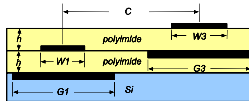
Fig. 3. Embedded finite-ground microstrip lines.
