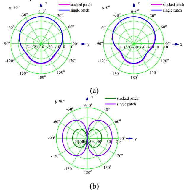
Fig. 9. Radiation pattern of the (a) copolarized and (b) cross-polarized component of the stacked patch antenna at 5.8 GHz.
