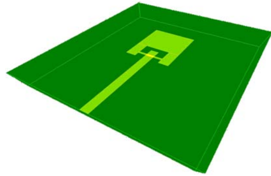
Fig. 6. MEMS switch feeding capacitive stub
