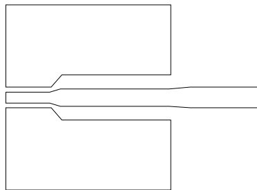
Fig. 1. CPW to microstrip transition
