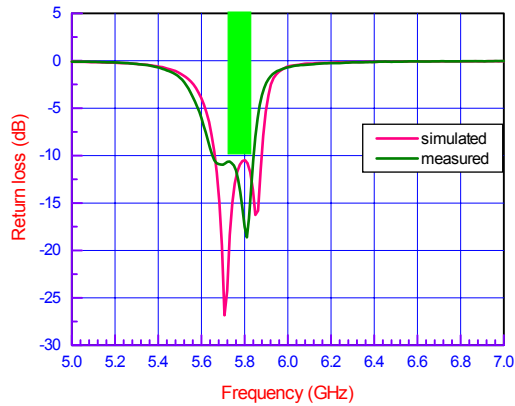
Fig. 8. Simulated and measured return loss of the stacked patch antenna for IEEE 802.11a 5.8 GHz band
