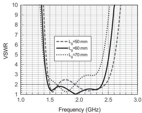
Fig. 3 Effect of the length ( L_g ) of the ground plane on the broadband performance of the quasiplanar antenna
