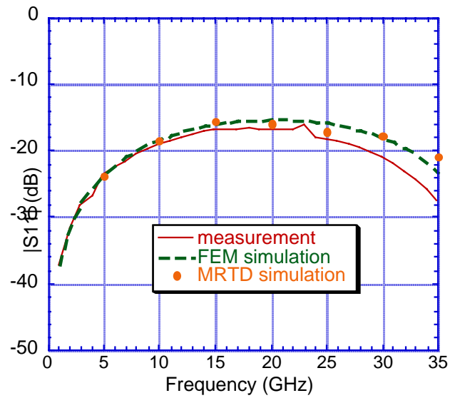
Fig.3 Verification with FEM and Test Structure Measurements
