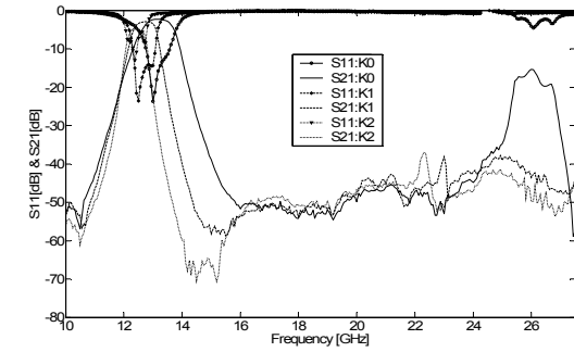
(c) 3-pole
