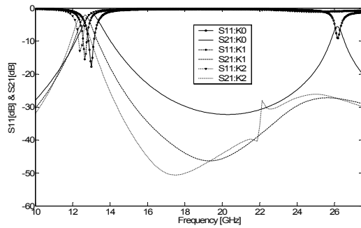
(a) 1-pole
