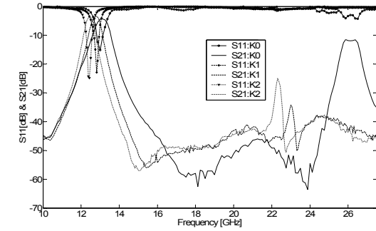
(b) 2-pole
