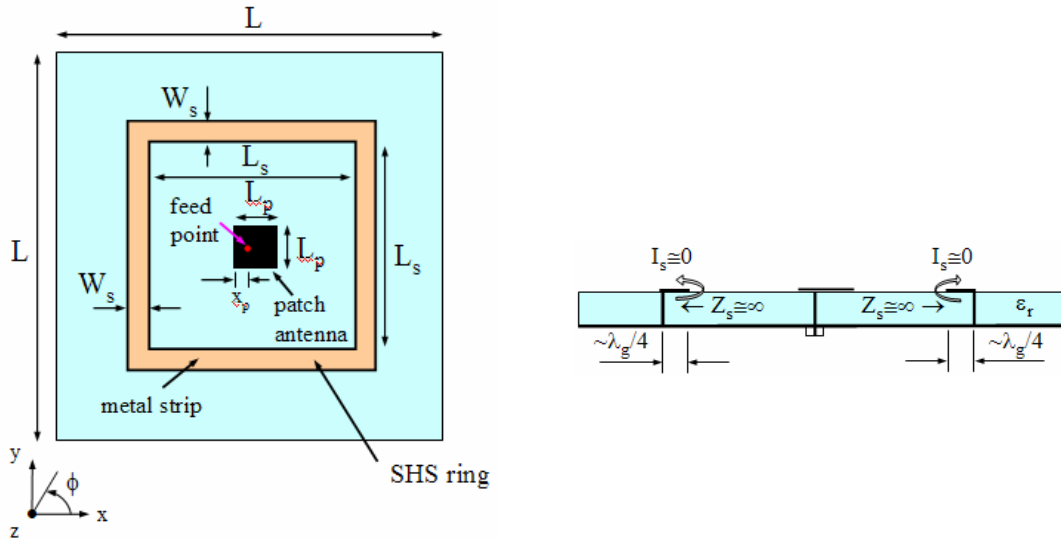
Figure 1. Stacked patch antenna surrounded by SHS structure.
